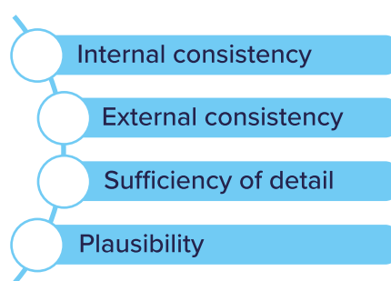
Figure 3. Credibility indicators
