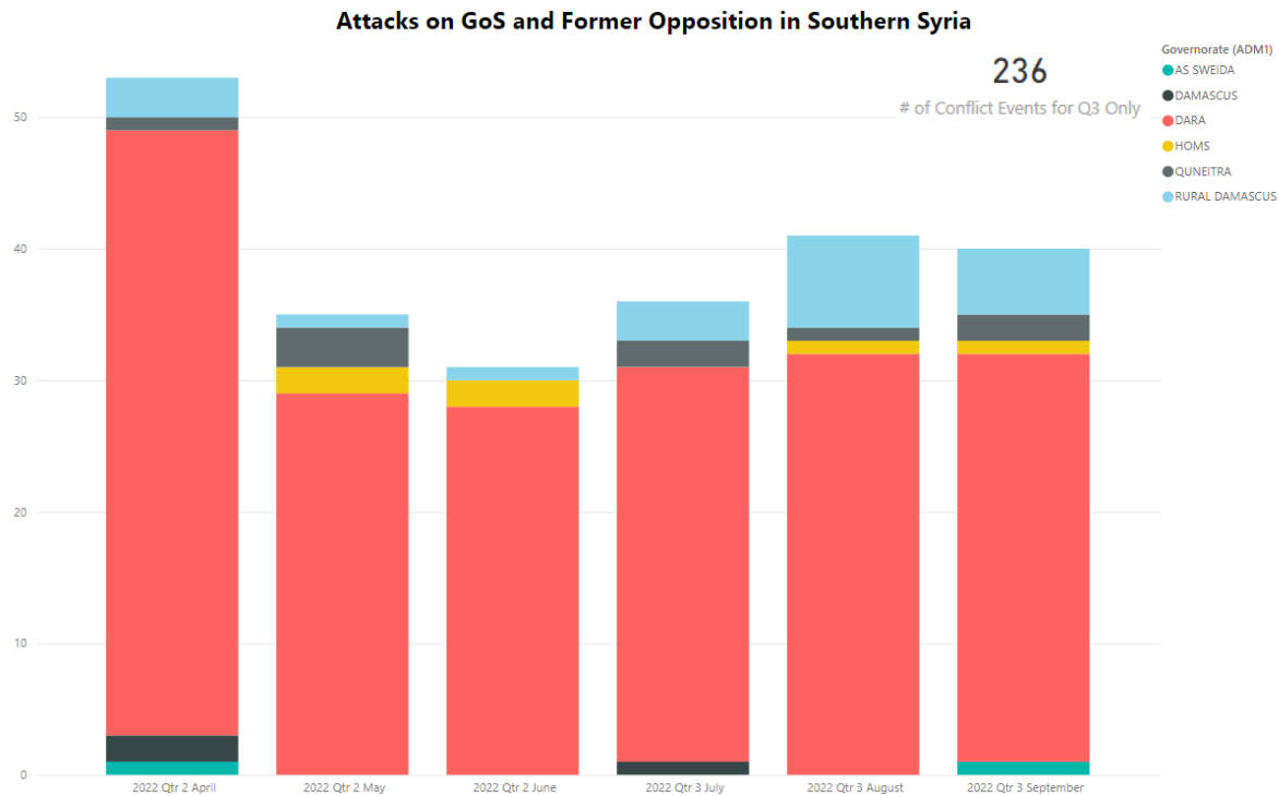
Figure 6: Attacks against former opposition fighters and GoS armed forces in southern Syria between April -September 2022. Data from The Carter Center and ACLED.
