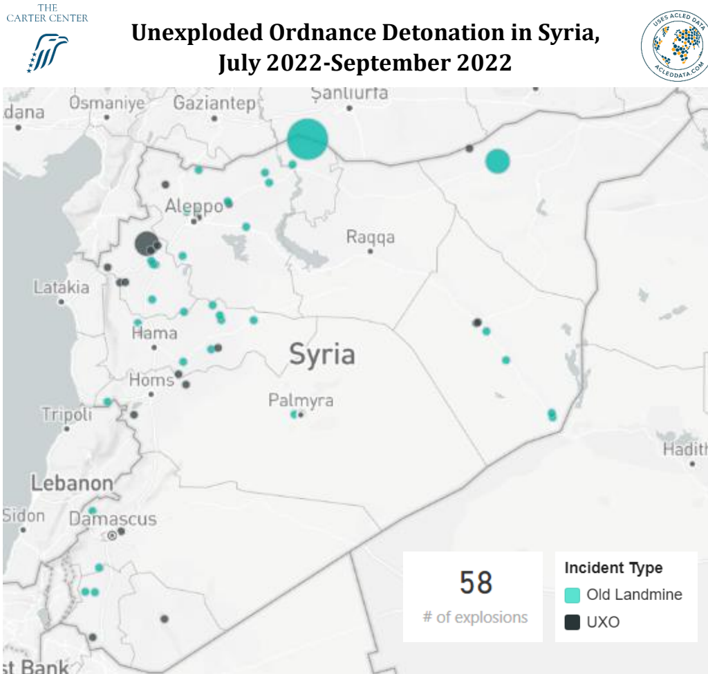
Figure 8: Detonations of old landmines and unexploded ordnance in Syria since July-September 2022. The largest bubble represents 3 detonation events. Data from The Carter Center and ACLED.
