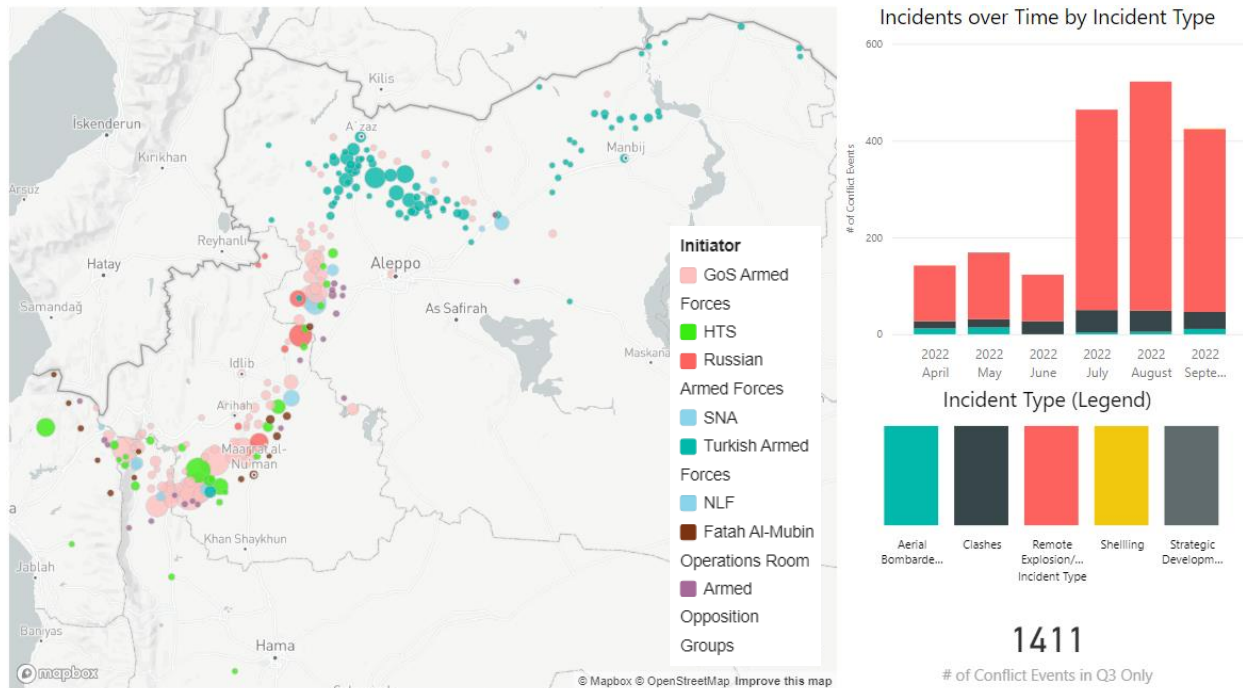
Figure 4: Conflict between GoS armed forces and armed opposition groups in northwest Syria from July through September 2022. The largest bubble represents 58 conflict events. Data from The Carter Center and ACLED.
