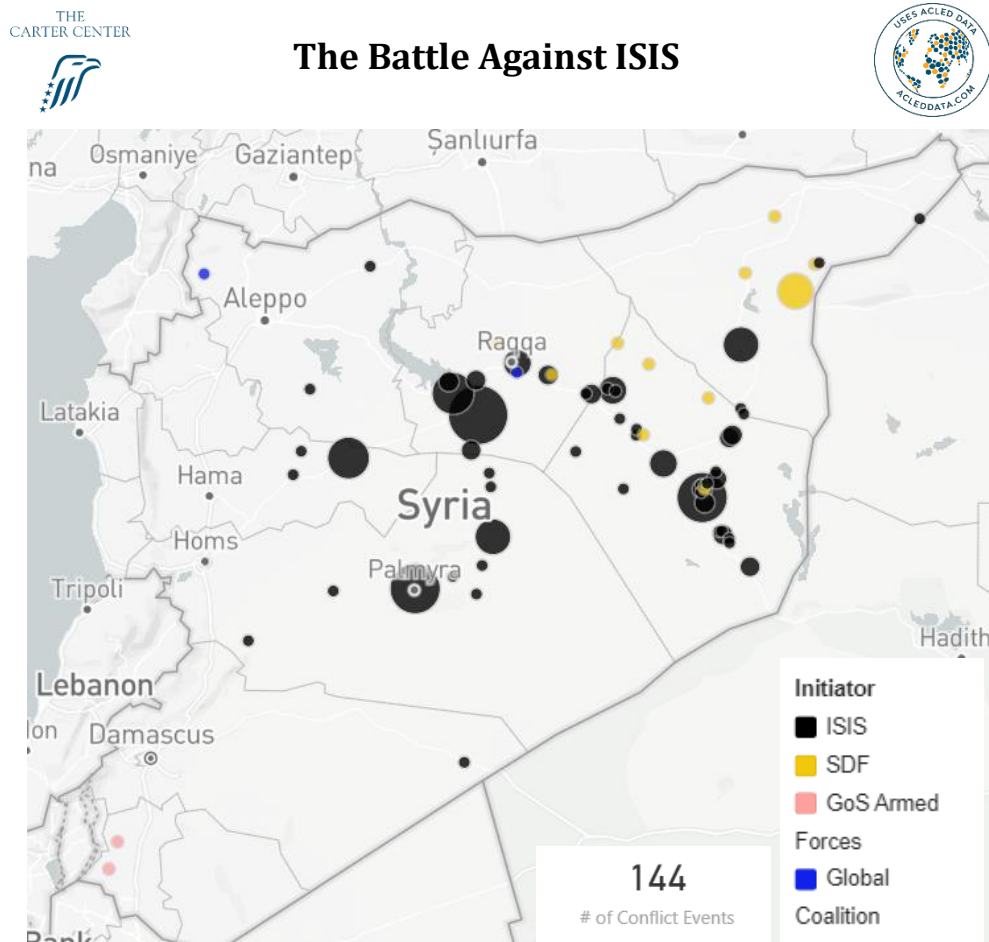
Figure 7: Incidents involving ISIS between July-September 2022. The largest bubble represents 25 conflict events. Data from The Carter Center and ACLED.
