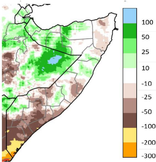
Difference in total rainfall (mm) received from 1 April to 30 June 2021 compared to the 1981 to 2020 average. Source: Climate Hazards Center, UC Santa Barbara
